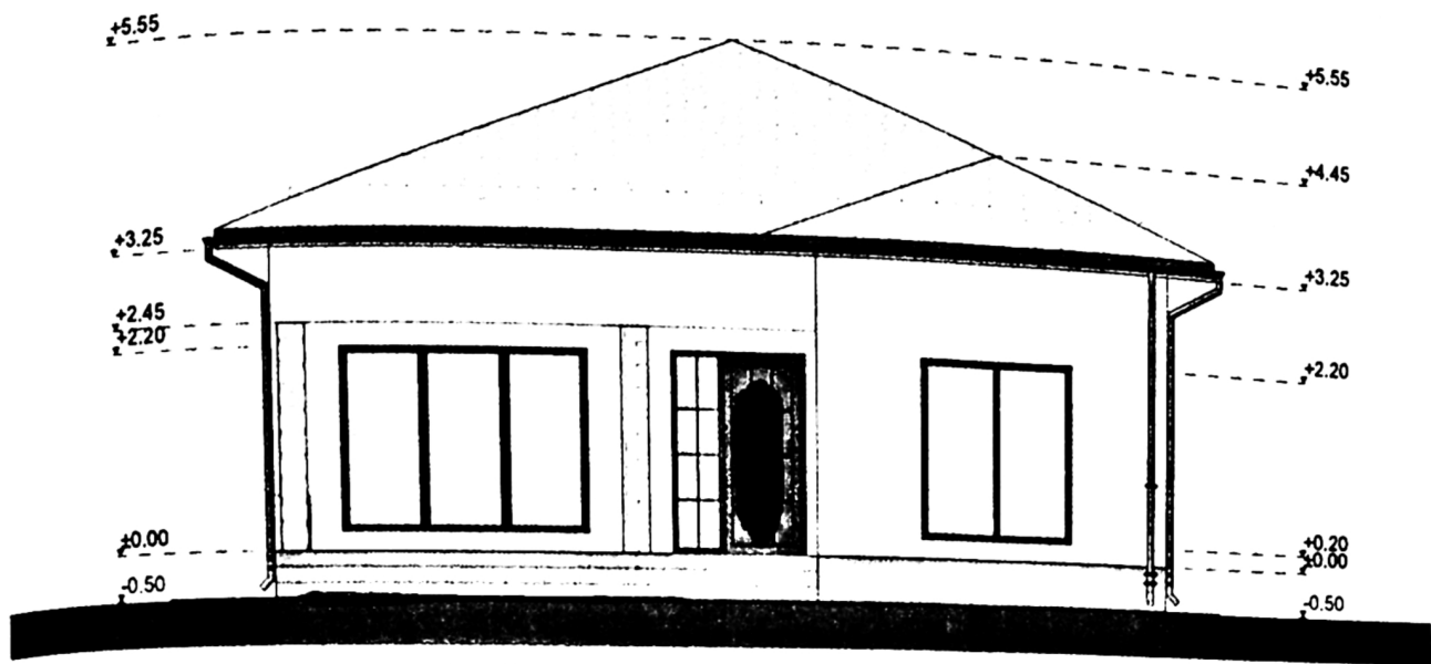
FATADA PRINCIPALA
